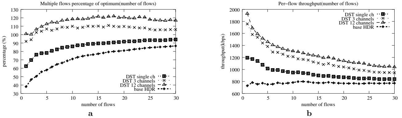
Fig. 10. (a) The throughput of DST and the basic cellular rate as percentage of the throughput achieved by Bellman-Ford when the number of flows grows from 1 to 30 for a network of 300 hosts. We show the results for DST run using 802.11b in single channel mode, 802.11b in 3-channel mode and 802.11a using all 12 channels. (b) The per-flow throughput corresponding to (a).
