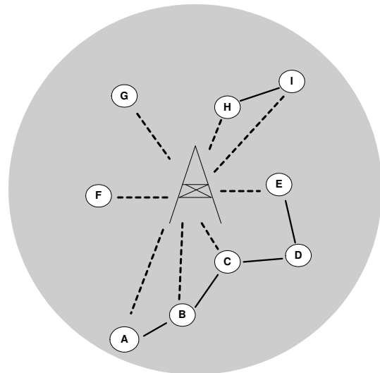
Fig. 1. Example of a multihop cellular network. The grey area represents the coverage cell of the base station. Dashed lines represent cellular links, and full lines represent Wi-Fi wireless links.
