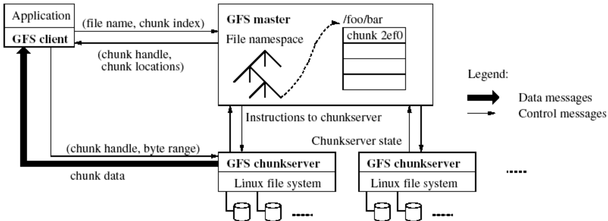
Figure 1: GFS Architecture
