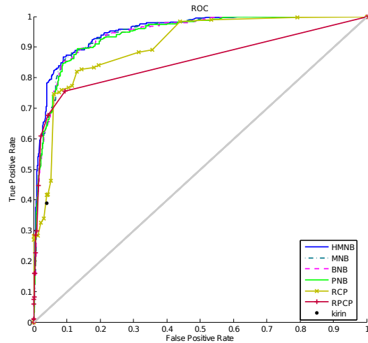
(a) ROC for the best performing parameters for each method.
