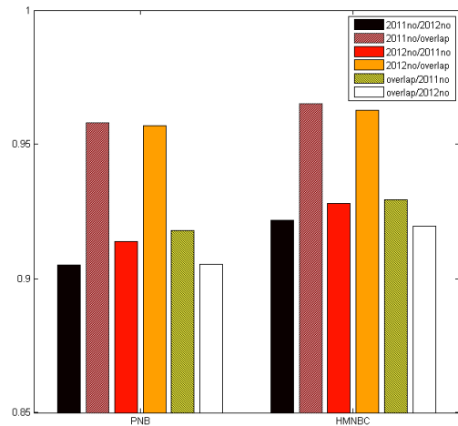
Figure 5: Comparison of 2011 and 2012 Data for PNB and HMNB models. ‘no’ = no overlap, ‘over’ = only overlap. ‘first/second’ means the first dataset was used to train, and the second dataset was used to test along with the malware. Then the AUC was generated and generated.
