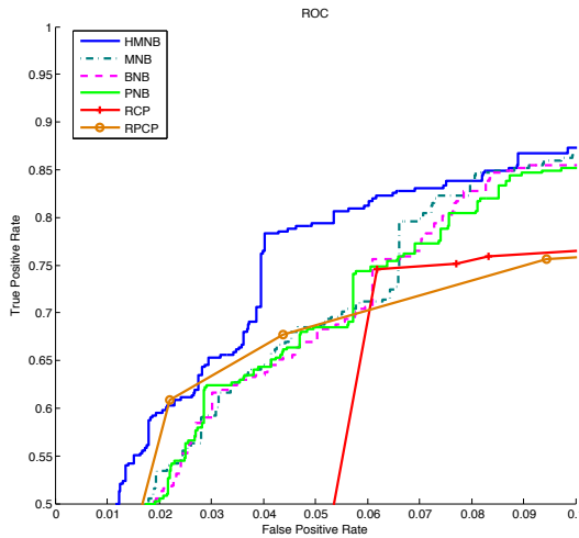
(b) Close up of Figure 3(a) to capture performance differences in the first 10% false positives
